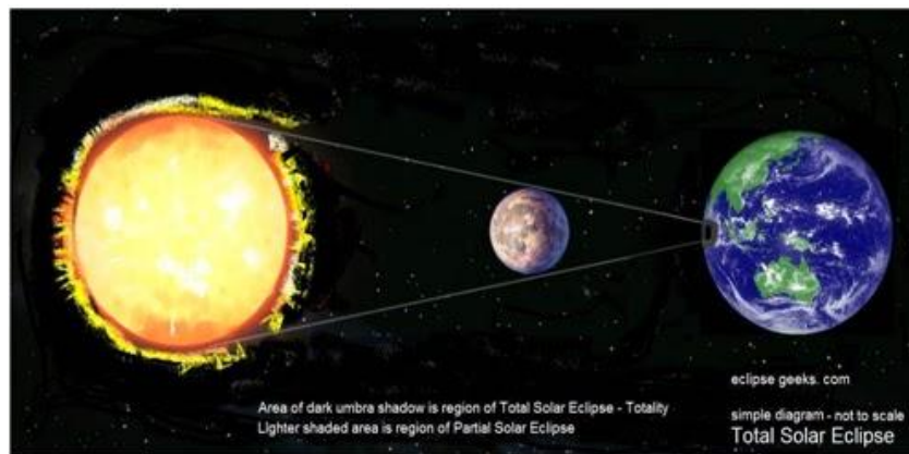
Gambar Gerhana Matahari
